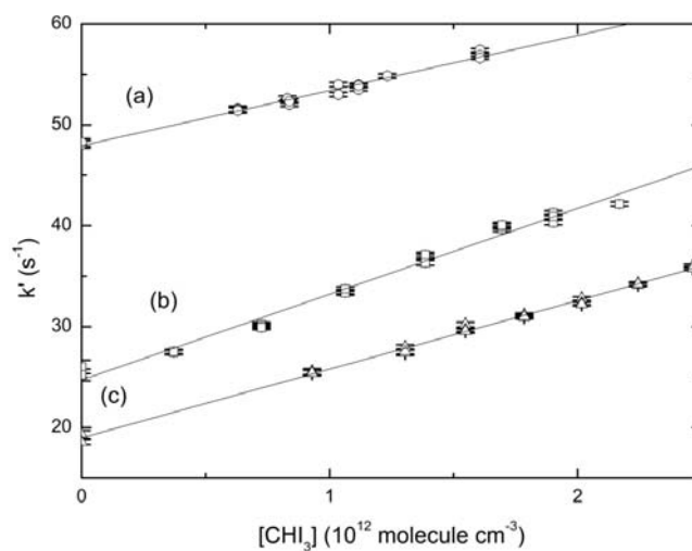
Fig. 4. Second order plots of k' versus [CHI_3] for the reaction (2) with O atoms at three different temperatures. Fits are obtained from linear least squares analyses and give the following bimolecular rate coefficients in units of 10^{-12} \text{ cm}^3 \text{ molecule}^{-1} \text{ s}^{-1} : (c) 6.8 \pm 0.16 at 298K, (b) 8.49 \pm 0.46 at 317K, (a) 5.46 \pm 0.36 at 373K. The error bars are 2\sigma statistical errors in k' .
