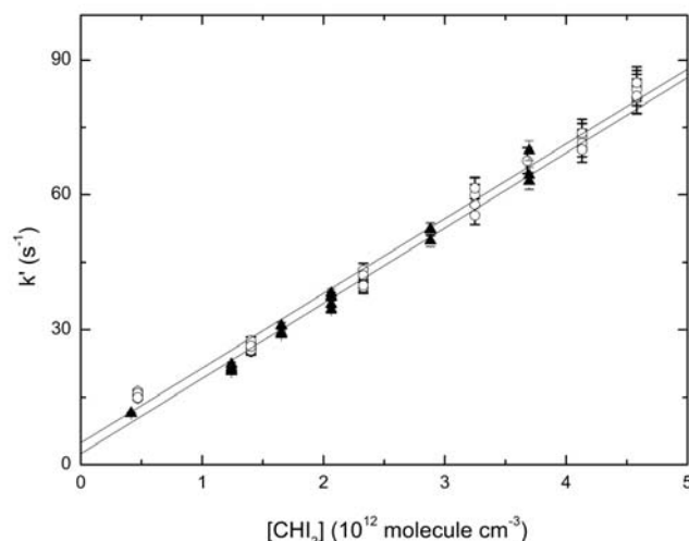
Fig. 5. Second order plots of k' versus [\text{CHI}_3] for the reaction (3) with OH radicals at 298K. Fits are obtained from linear least squares analyses and give the following bimolecular rate coefficients in units of 10^{-11} \text{ cm}^3 \text{ molecule}^{-1} \text{ s}^{-1} : (○) 1.67 \pm 0.06 (▲) 1.66 \pm 0.06 . The error bars are 2\sigma statistical errors in k' .
