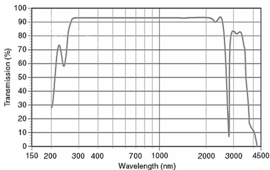
Figure V- 3 : Spectre 15 de transmittance du Quartz
