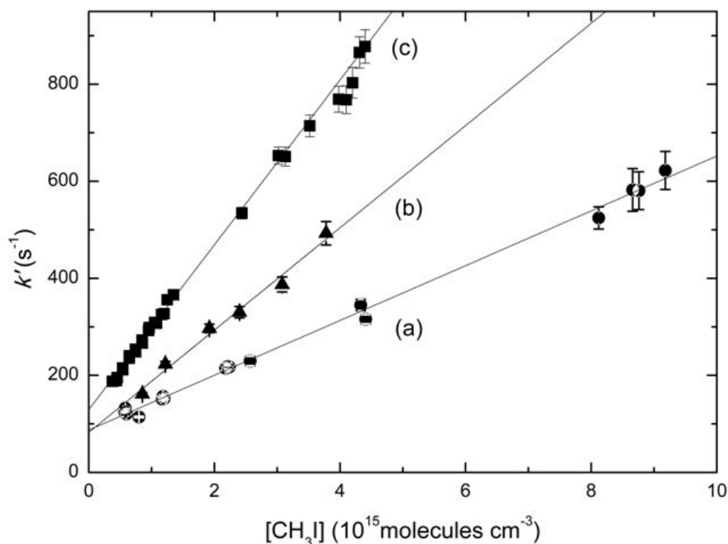
Fig. 3. Plots of k' versus [\text{CH}_3\text{I}] for data obtained at three different temperatures. Fits are obtained from linear least squares analyses and give the following bimolecular rate coefficients in units of 10^{-14} \text{ cm}^3 \text{ molecule}^{-1} \text{ s}^{-1} : (a) 5.72 \pm 0.17 at 295 K, (b) 10.5 \pm 1.3 at 323 K, and (c) 16.7 \pm 0.6 at 390 K.
