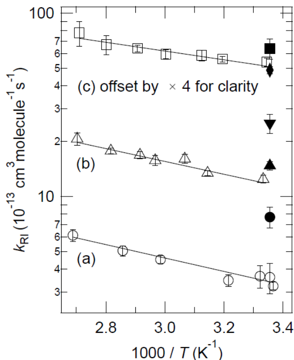
Fig. 6 Arrhenius plot for the reaction OH + C 2 H 5 I (a), OH + n-C 3 H 7 I (b) and OH + iso-C 3 H 7 I (c) obtained in this work. The solid lines are Arrhenius expressions fitted to the rate constants k_{RI} obtained in this work. The uncertainties are \pm 2\sigma , as returned by weighted, (1/\sigma^2) , least squares fitting to data listed in Table 1. Data points \bullet , \blacktriangledown and \blacksquare , were taken from Cotter et. al. (2003) 25 and correspond to room temperature reactions OH + C 2 H 5 I, OH + n-C 3 H 7 I and OH + iso-C 3 H 7 I, respectively. Data points \blacklozenge and \blacktriangle were taken from Carl and Crowley (2001) 11 and correspond to room temperature reactions OH + n-C 3 H 7 I and OH + iso-C 3 H 7 I, respectively.
