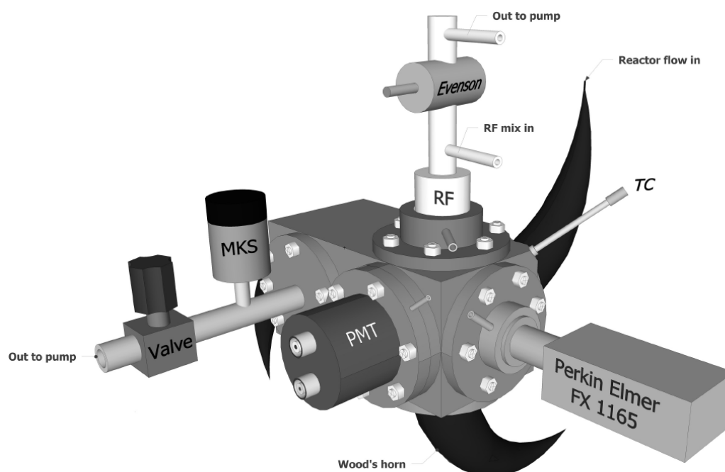
Fig.1 Schematic representation of the Flash Photolysis Resonance Fluorescence (FPRF) apparatus used to study the reaction of OH radicals with CHI_3 and these of O atoms with C_2H_5I , and CHI_3 . RF: Resonance Fluorescence Lamp; Evenson: Evenson microwave cavity; MKS: MKS 1000 Torr Capacitance Manometer; PMT: Photomultiplier tube; TC: Type J thermocouple
