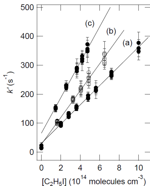
Fig. 3 Plots of k' versus [C_2H_5] for data obtained at three different temperatures. Fits are obtained from linear least squares analyses and give the following bimolecular rate coefficients in units of 10^{-13} molecule cm^3 s^{-1} : (a) 3.24 \pm 0.08 at 297K, (b) 4.52 \pm 0.11 at 335K, (c) 6.13 \pm 0.23 at 372K. The error bars are 2\sigma statistical errors in k' .
