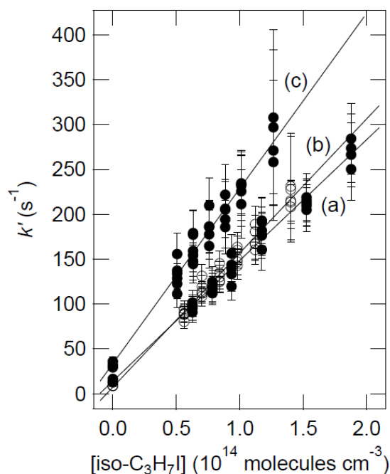
Fig. 5 Plots of k' versus [\text{iso-C}_3\text{H}_7\text{I}] for data obtained at three different temperatures. Fits are obtained from linear least squares analyses and give the following bimolecular rate coefficients in units of 10^{-13} molecule \text{cm}^3 \text{s}^{-1} : (a) 13.5 \pm 0.7 at 299K, (b) 14.9 \pm 0.8 at 333K, (c) 19.5 \pm 3.0 at 369K. The error bars are 2\sigma statistical errors in k' .
