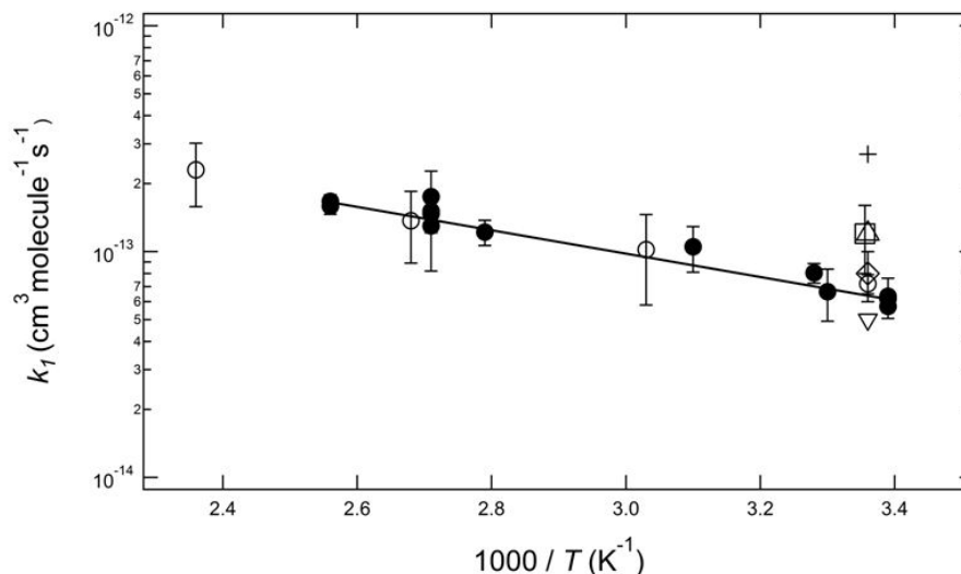
Fig. 4. Comparison of the Arrhenius plots for the reaction of OH with CH 3 I obtained in this work (●); Brown et al. (○); Gilles et al. , (□); Cotter et al. (◇); Garraway (+); Marshall et al. using Møller-Plesset frequency calculations (△) and Hartree-Fock frequency calculations (▽). The solid line is Arrhenius expression fitted to the rate constant k_1 obtained in this work.
