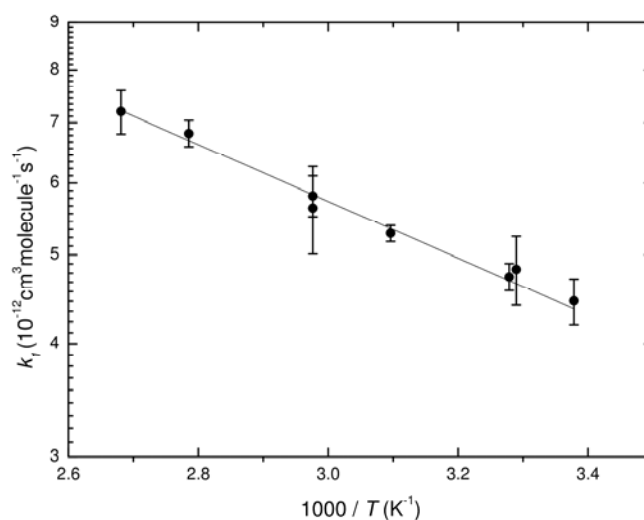
Fig. 4: Arrhenius plot for the reaction of OH with CH 2 I 2 obtained in this work. The solid line is Arrhenius expression fitted to the rate constant k_1 obtained in this work.
