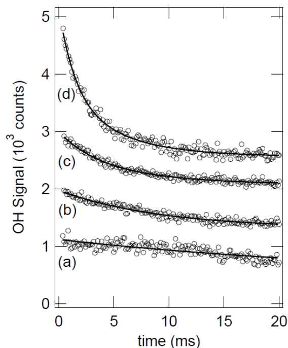
Fig. 2 Typical OH radical decay profiles as a function of [C_2H_5] . Experimental conditions: T = 297\text{ K} ; [H_2O] = 1.53 \times 10^{15}\text{ cm}^{-3} ; [C_2H_5] in units of 10^{14}\text{ cm}^{-3} : (a) 0 (b) 2.01; (c) 4.81; (d) 10.0. Number of flashes averaged = 60 each for traces (a) to (d). The quantity plotted in the y-axis is total accumulated signal counts, which is proportional to the number of lamp flashes averaged and the multichannel scalar dwell time ( 122\text{ }\mu\text{s} per channel in all traces shown). Solid lines are obtained from least-squares analyses that give the following best fit parameters k' in units of \text{s}^{-1} : (a) 14 (b) 91; (c) 186; (d) 359. The plots have been displaced vertically for clarity.
