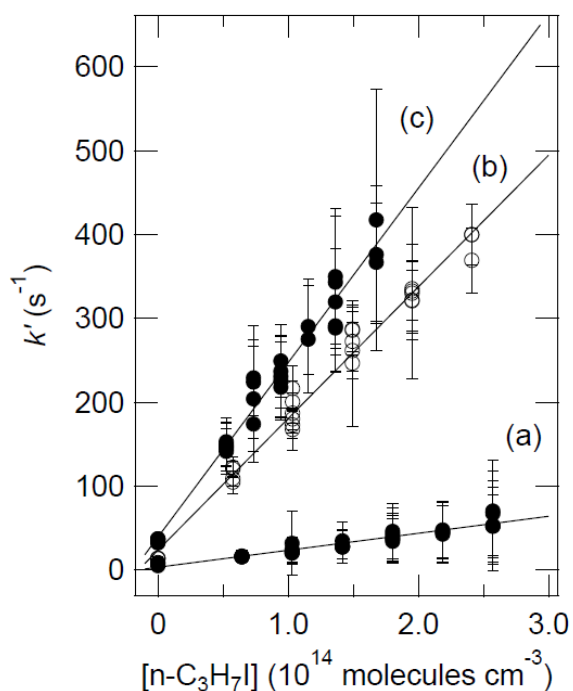
Fig. 4 Plots of k' versus [n-C_3H_7] for data obtained at three different temperatures. Fits are obtained from linear least squares analyses and give the following bimolecular rate coefficients in units of 10^{-13} molecule cm^3 s^{-1} : (a) 12.4 \pm 0.06 at 300K, (b) 15.7 \pm 1.0 at 337K, (c) 20.6 \pm 1.6 at 370K. The error bars are 2\sigma statistical errors in k' .
