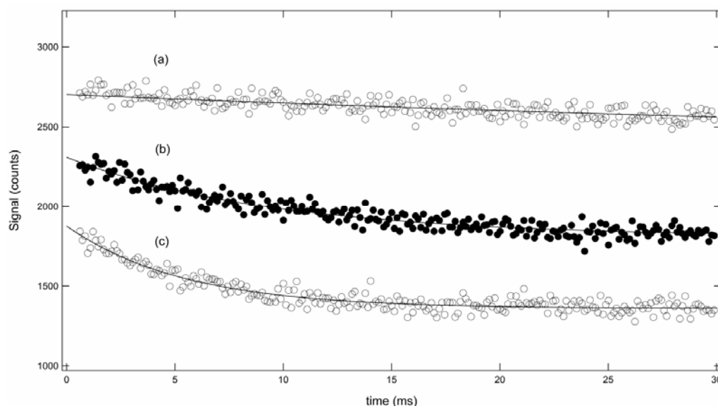
Fig. 2. Typical OH decay temporal profiles observed in studies of reaction (1) employing 187 Torr of He buffer gas. Experimental conditions: T = 303 \text{ K} ; [\text{H}_2\text{O}] = 2.11 \times 10^{15} \text{ molecules cm}^{-3} ; [\text{CH}_3\text{I}] = in units of 10^{15} \text{ molecules cm}^{-3} = (a) 0, (b) 0.84, (c) 16.7. Number of flashes = (a) 200, (b) 200, (c) 200. Solid lines are obtained from least squares analyses that give the following best fit parameters (considering the Poisson distribution of the counts): k' in units of \text{s}^{-1} (a) 14, (b) 106, (c) 186. The plots have been displaced vertically for clarity.
