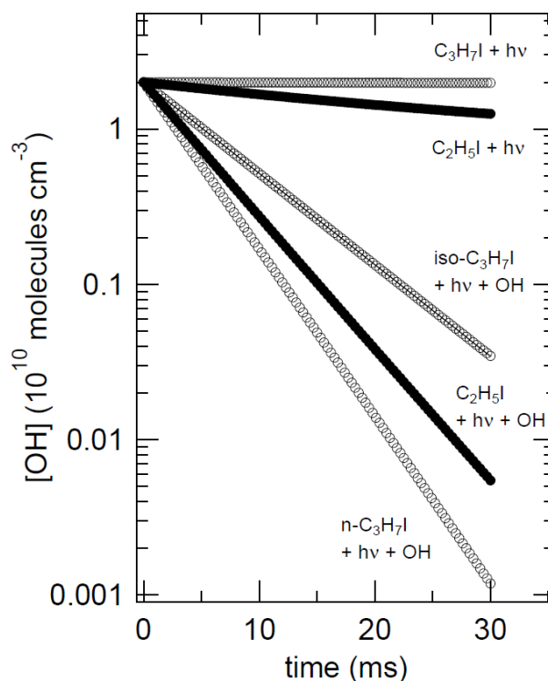
Fig. 7 Model results for potential loss of C_2H_5I , n-C_3H_7I and iso-C_3H_7I due to VUV photolysis to produce C_2H_5 and C_3H_7 radicals and I atoms. Initial I atom, C_2H_5 and C_3H_7 radical concentrations were calculated using equation VIII. ( C_2H_5I+h\nu ): Modeled OH radical consumption calculated using reactions (6), (7)-(12), and (20)-(26) listed in Table 3 that results is the calculated decay rate of 31s^{-1} . ( C_2H_5I+h\nu+OH ) Modeled OH radical consumption calculated using reaction (1) in addition to reactions (6), (7)-(12), and (20)-(26) listed in Table 3 that results in the calculated decay rate of 199s^{-1} . The decay rate ratio yields a 16% difference in the OH radical consumption due to VUV photolysis of C_2H_5I ; ( C_3H_7I+h\nu ): Modeled OH radical consumption calculated using reactions (6), (7)-(12), and (20)-(26) listed in Table 3 that results in the calculated decay rate of 31s^{-1} . ( iso-C_3H_7I+h\nu+OH ): Modeled OH radical consumption calculated using reaction (3) in addition to reactions (6), (13)-(18), and (20)-(26) listed in Table 3 that results in the calculated decay rate of 135s^{-1} . The decay rate ratio yields a 11% difference in the OH radical consumption due to VUV photolysis of iso-C_3H_7I ; ( n-C_3H_7I+h\nu+OH ): Modeled OH radical consumption calculated using reaction (2) in addition to reactions (6), (13)-(18), and (20)-(26) listed in Table 3 that results is the calculated decay rate of 247s^{-1} . The decay rate ratio yields a 6% difference in the OH radical consumption due to VUV photolysis of n-C_3H_7I .
