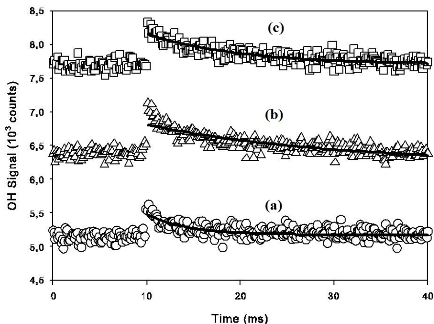
Fig. 2. Typical OH radical decay profiles as a function of [\text{CHI}_3] . Experimental conditions: T = 298 \text{ K} ; [\text{H}_2\text{O}] = 1.52 \times 10^{15} \text{ cm}^{-3} ; [\text{CHI}_3] in units of 10^{12} \text{ cm}^{-3} : (a) 0 (b) 2.32; (c) 4.58. Decays are averaged from 200 flashes each for traces (a) to (c). The quantity plotted on the y-axis is total accumulated signal counts, which is proportional to the number of lamp flashes averaged and the multichannel scaler dwell time ( 122 \mu\text{s} per channel in all traces shown). Solid lines are obtained from least-squares analyses that give the following best fit parameters k' in units of \text{s}^{-1} : (a) 10 \pm 0.6 (b) 39 \pm 2 ; (c) 84 \pm 6 . The plots of curves (b) and (c) have been displaced vertically for clarity.
