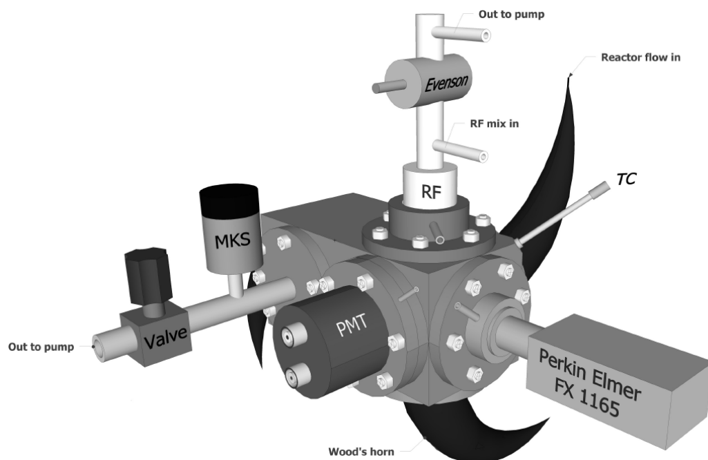
Fig. 1 Schematic representation of the Flash Photolysis Resonance Fluorescence (FPRF) apparatus used to study the reaction of OH radicals with C_2H_5I , n-C_3H_7I and iso-C_3H_7I . RF: Resonance Fluorescence Lamp; Evenson: Evenson microwave cavity; MKS: MKS 1000 Torr Capacitance Manometer; PMT: Photomultiplier tube; TC: Type J thermocouple
