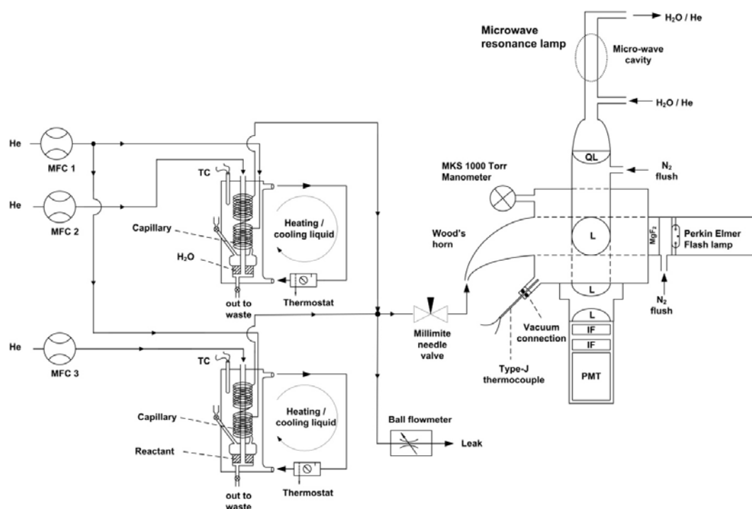
Fig. 1. Schematic representation of the Flash Photolysis Resonance Fluorescence apparatus used to study the reaction of OH radicals with \text{CH}_3\text{I} . PMT: photomultiplier tube; L: quartz lenses anti-reflection coated for 308 nm; IF: 308 nm Interference filters; QL: quartz lens; MCF: mass flow controller; TC: Type J thermocouple
