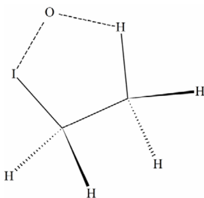
Fig. 7. Schematic representation of a five-membered cyclic transition state in the reaction of O(^3P) with \text{C}_2\text{H}_5\text{I} and the HOI product molecule. Figure adapted from Reid et al. (2000). 40
