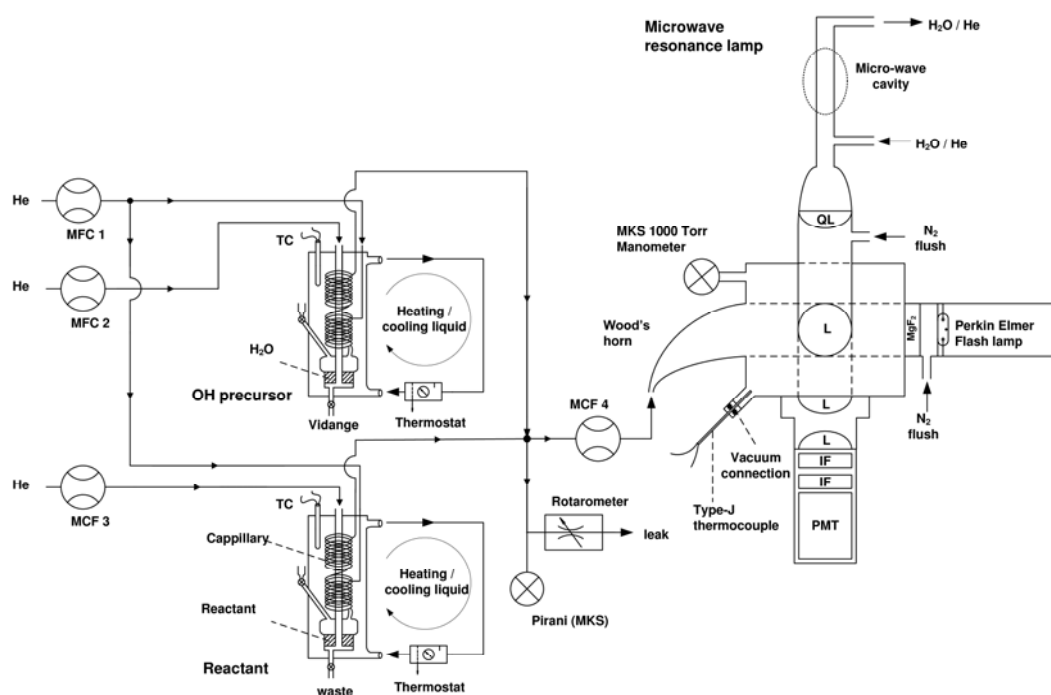
Fig. 1: Schematic representation of the Flash Photolysis Resonance Fluorescence apparatus used to study the reaction of OH radicals with \text{CH}_2\text{I}_2 . PMT: Photomultiplier tube; L: Quartz lenses anti-reflection coated for 308 nm; IF: 308 nm interference filters; QL: Quartz lens; MCF: Mass flow controller; TC: Type J thermocouple
